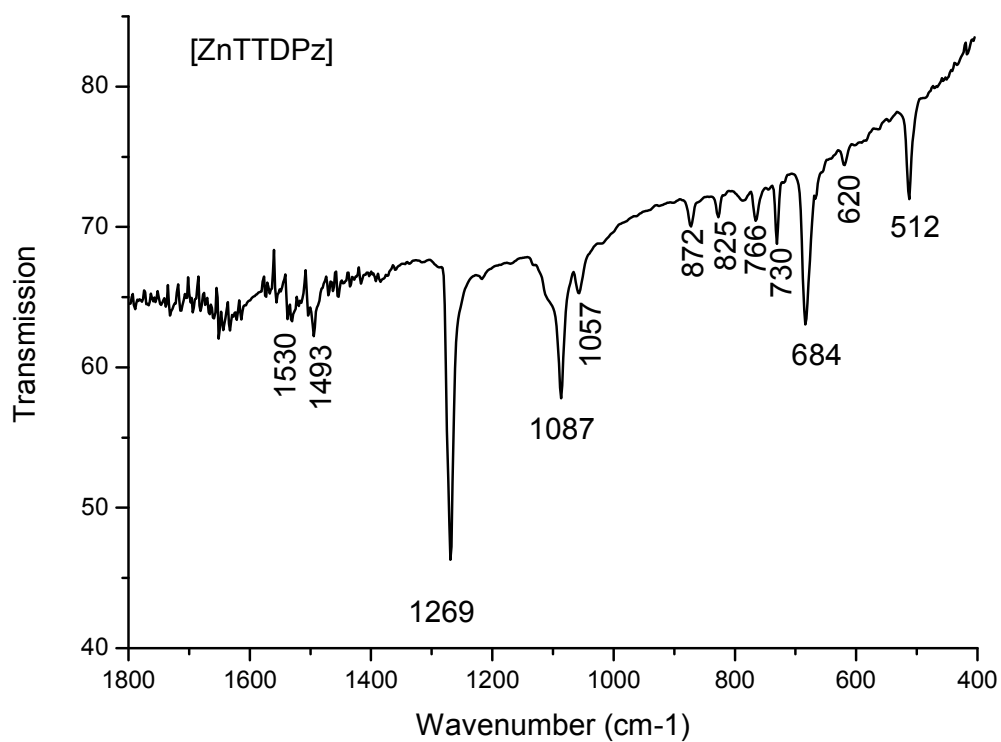
Figure S2. IR spectrum of [ZnTTDPz] (solid film).
