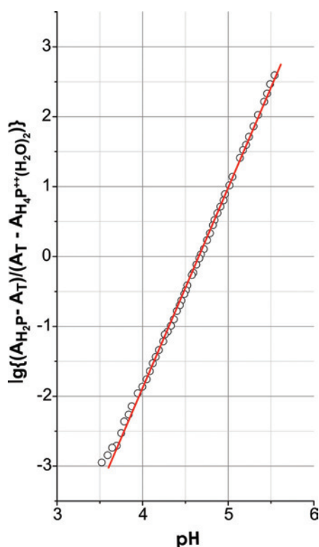
Figure 5. Dependence of \lg(I_n) on pH for H_2P(PhSO_3^-)_4 in system (I).
