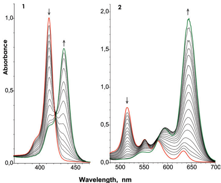
Figure 2. UV-vis spectra of system (I) at pH = 2-8 , at porphyrin concentration 2.07 \cdot 10^{-5} mol/l (1) and 1.23 \cdot 10^{-4} mol/l (2): \downarrow H_2P(PhSO_3^-)_4 , \uparrow [H_4P^{2+}(PhSO_3^-)_4](H_2O)_2 .
