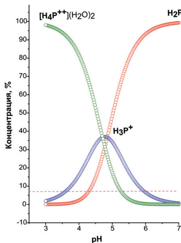
Figure 6. Distribution of equilibrium concentrations of H_2P , H_3P^+ and [H_4P^{2+}](H_2O)_2 in system (I).
