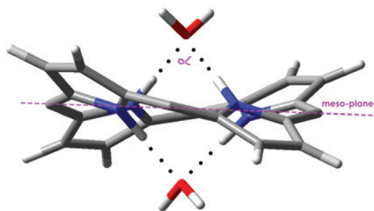
Figure 1. Geometry of solvatocomplex [H_4P^{2+}(PhSO_3^-)_4](H_2O)_2 (phenyl rings are not shown).
